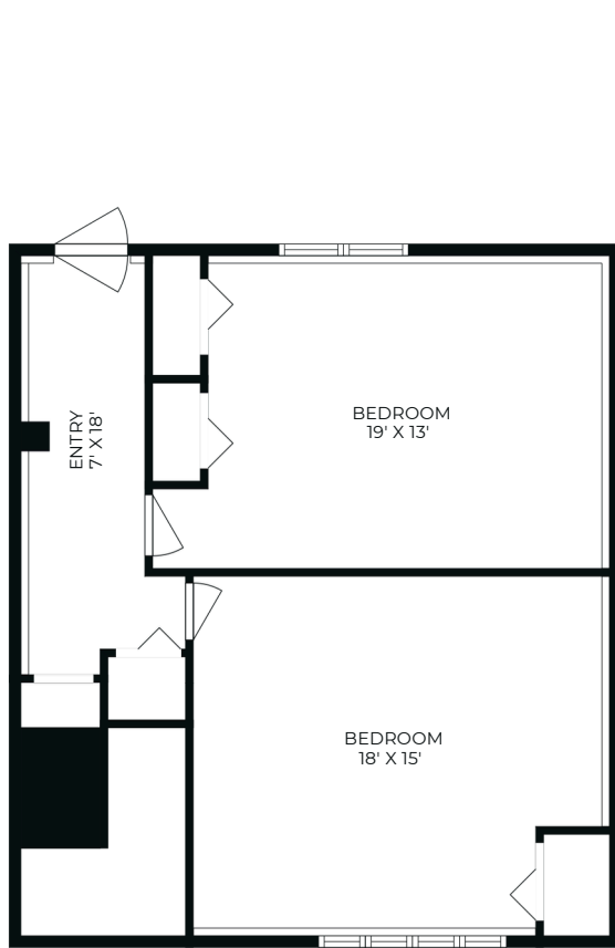
FLOOR 1
